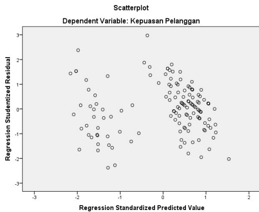
Gambar 4. Scatterplot
