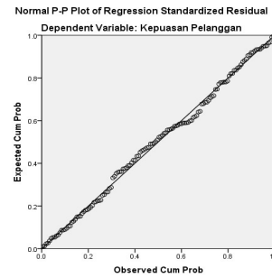
Gambar 3. P-Plot Of Reprssion Standardized Residual
